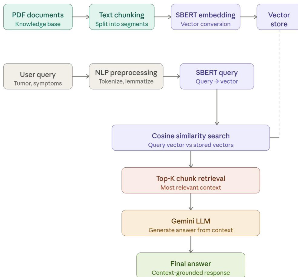
Figure 3.5 : RAG workflow in NeuroVision System
