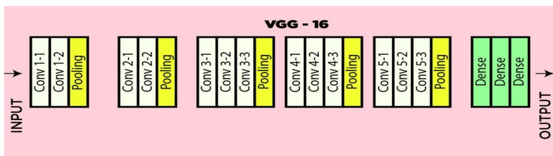
Figure 3.3 : Architecture of VGG-16
