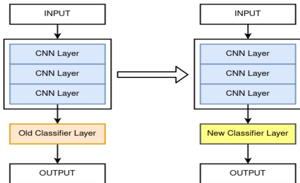
Figure 2.6 : Transfer Learning
