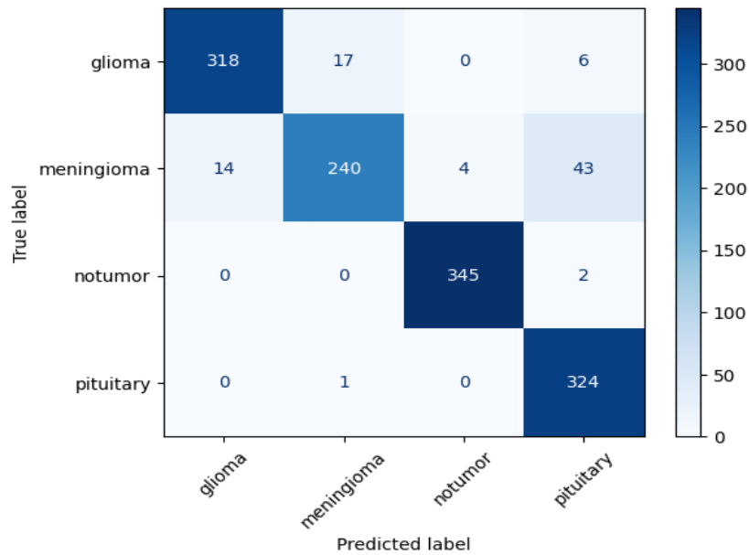
Figure 3.12: Confusion Matrix on Hospital Validation Dataset
